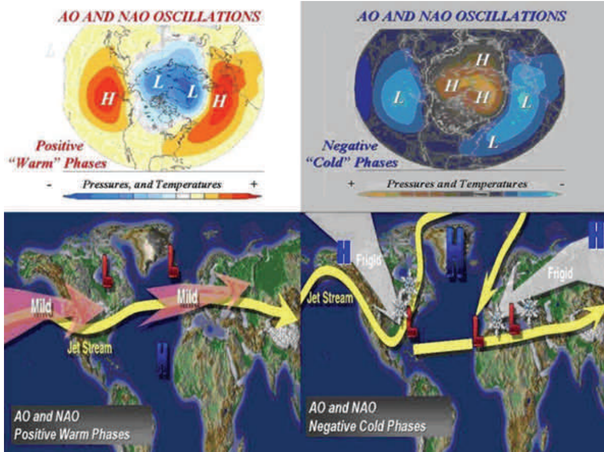
Figure 12. The Positive and Negative Phases of the AO and NAO (icecap.us).
