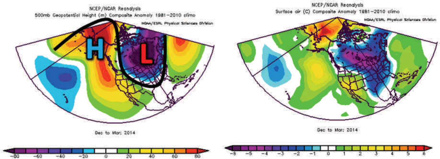
Figure 11. Jet stream pattern during the winter 2013-14 (left), and the surface temperature anomalies (right).
