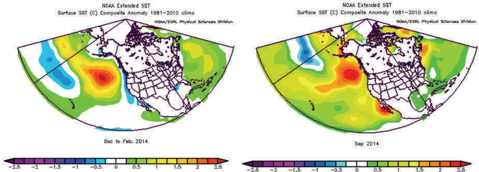
Figure 8. Sea Surface Temperature (SST) anomalies across the Pacific and Atlantic during the winter 2013-14 (September 2014) left (right).
