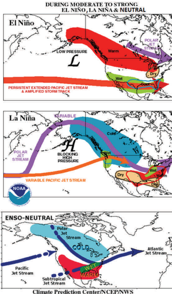
Figure 2. The typical upper level jet stream/storm track during El Niño (top), La Niña (middle) and Neutral (bottom) winters. Courtesy of NOAA, Climate Prediction Center
