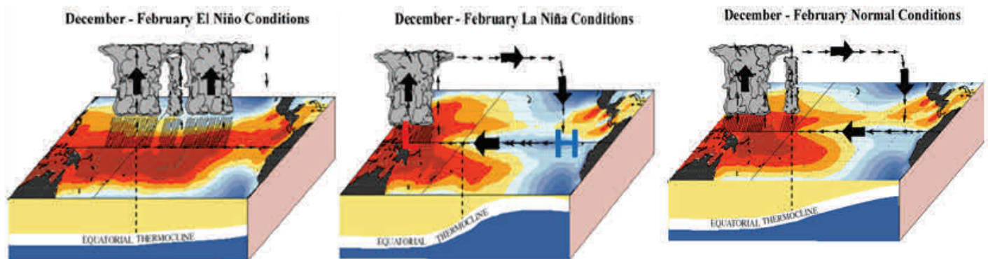
Figure 1 . The typical winter season conditions across the equatorial Pacific observed during El Niño (left) and La Niña (center) and Neutral (right).
