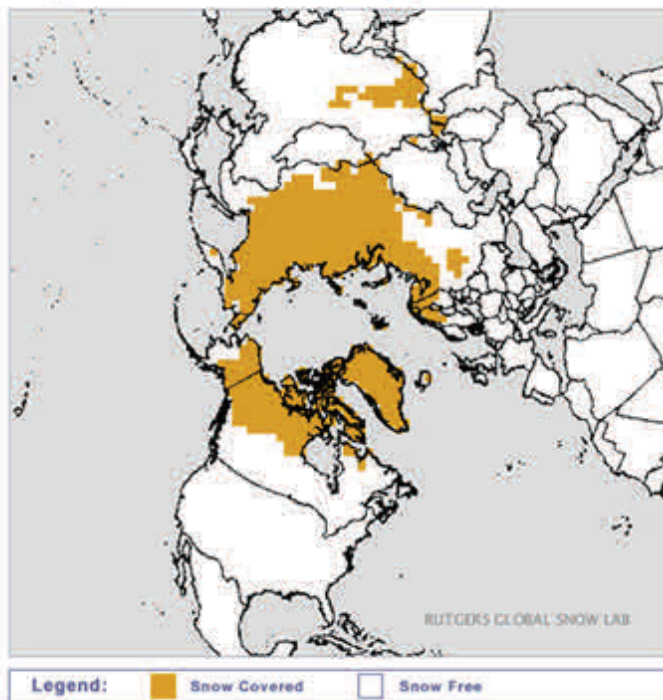
Figure 13. Current Northern Hemisphere snow cover as of October 18 th , 2014 (left), and the departure from normal (right). Courtesy Rutgers Global Snow Lab
