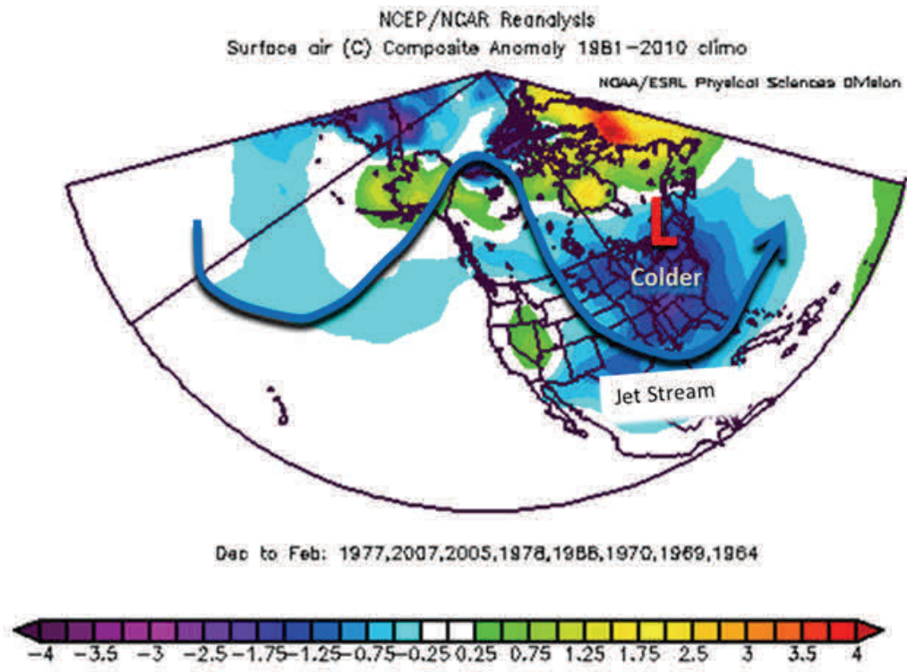
Figure 6. Same as figure 5 except during weak El Niño events.
