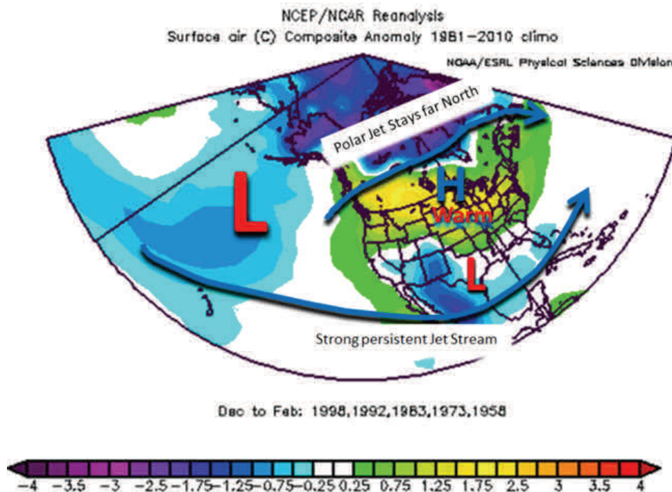
Figure 5. Composite map showing winter seasons during strong El Niño events. The blue arrows show the main placements of the upper level jets and the warm (cool) colors indicate positive (negative) temperature anomalies.
