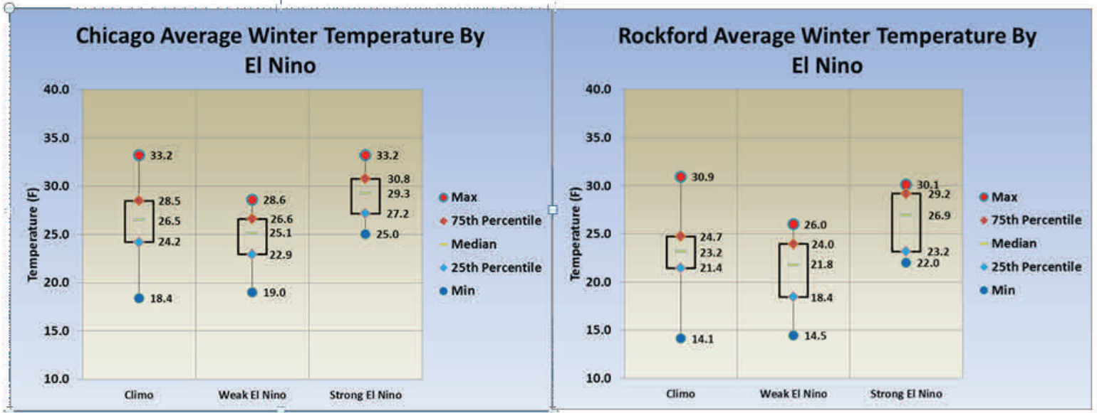
Figure 7. Box and Whisker plots showing the distributions of winter season (December through February) temperatures during weak and strong El Niño events relative to Climatology at Chicago, IL (left) and Rockford, IL (right).
