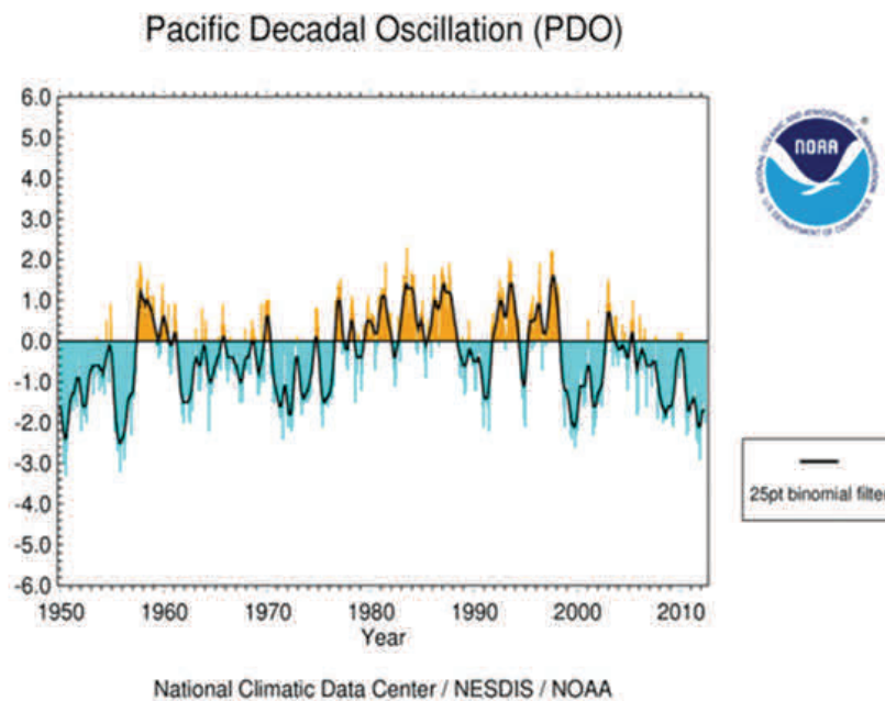
Figure 9. Behavior of the Pacific Decadal Oscillation (PDO) since 1950.
