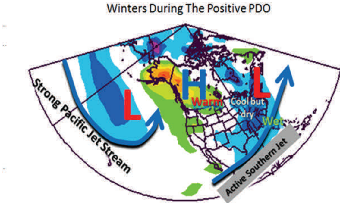
Figure 10. Typical winter season conditions during the positive PDO. The large blue arrow indicates the approximate placement of the Jet.
