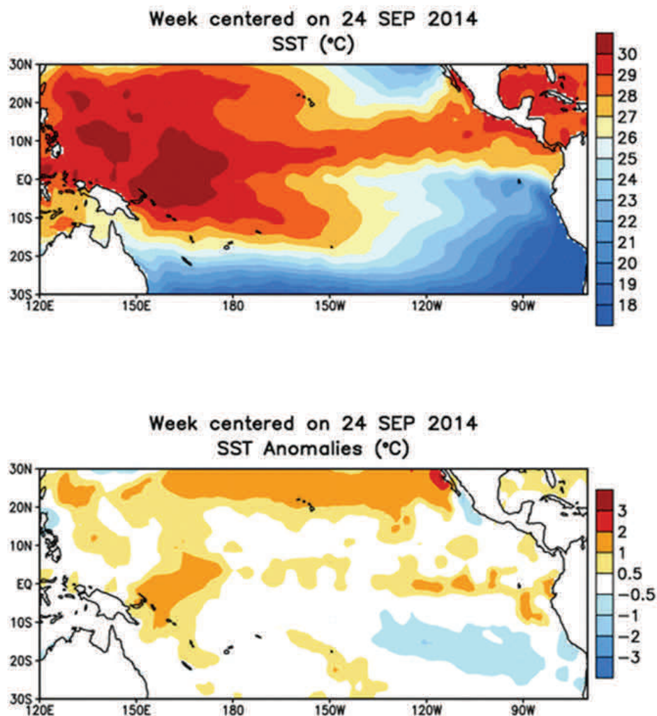
Figure 3 Observed sea surface temperatures across the equatorial Pacific (top) and their departures from average (bottom). Courtesy of NOAA, Climate Prediction Center
